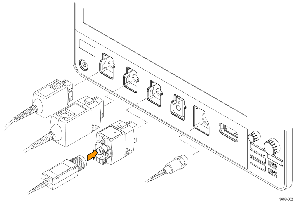
Figure 2: Connecting probes to the instrument
